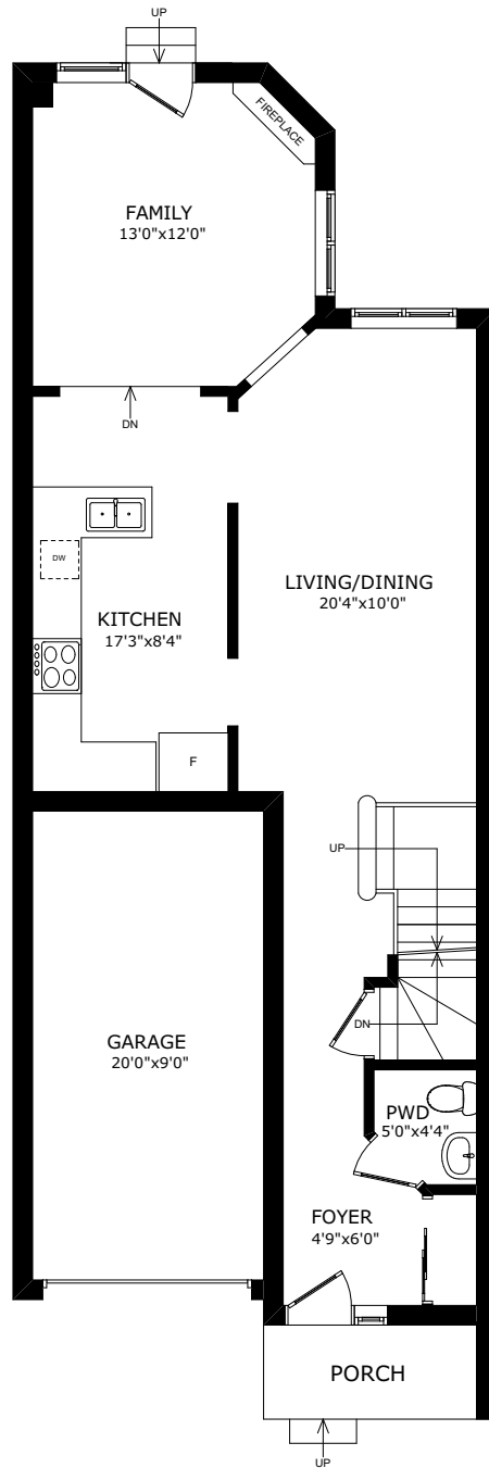
MAIN FLOOR
