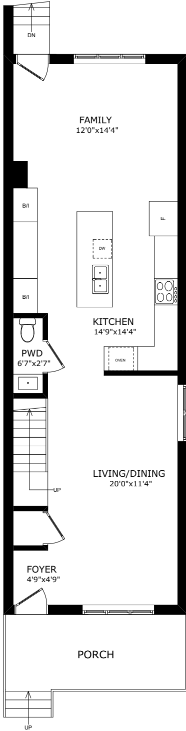
MAIN FLOOR
