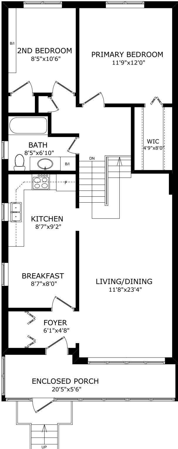
MAIN FLOOR
